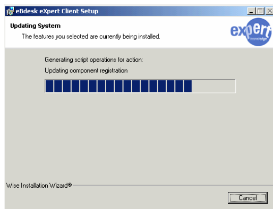
Gambar 1 - 6: Proses Instalasi
